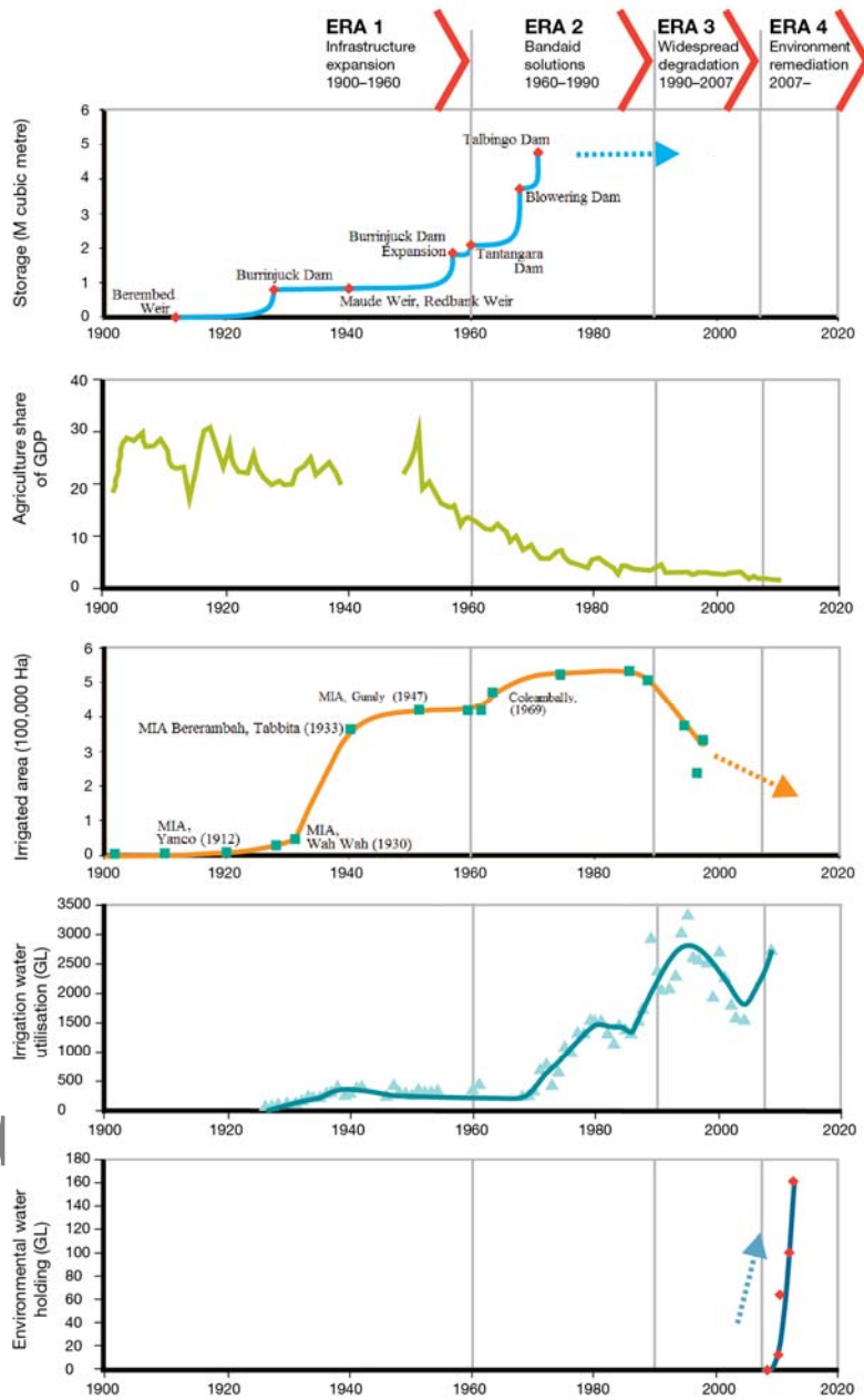
Figure 3: Pendulum Swing in the Murrumbidgee Basin. Time series of (a) storage, (b) agriculture's share of GDP, (c) irrigated area, (d) irrigation water use, and (e) environmental water holding.
